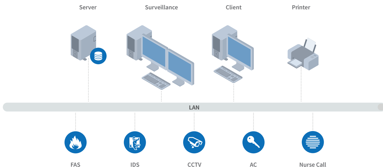
WinGuard system schematic
