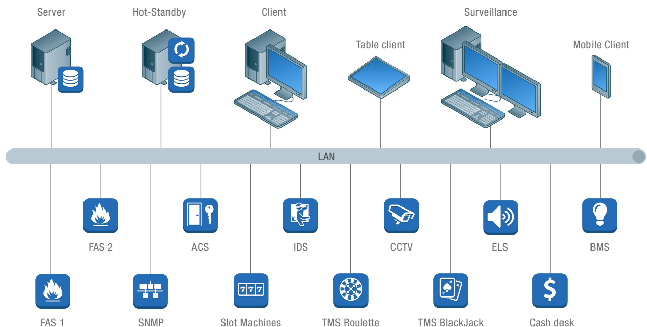
WinGuard system schematic
